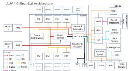
Fig. 7: Communication architecture block diagram.
