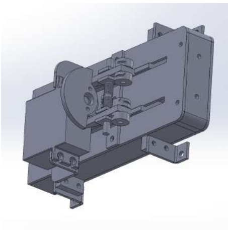
Fig. 6: BBAUV 4.0 Torpedo Launcher.
