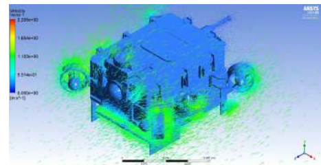
Fig. 12: Flow analysis in Ansys Fluent.
