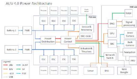
Fig. 8: Power architecture block diagram.
