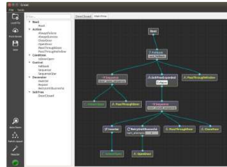
Fig. 10: Sample BT-based mission plan.
