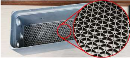
Fig. 5: Isogrid layer of the battery hulls.
