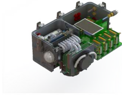
Fig. 3: Internal layout of the main hull.
